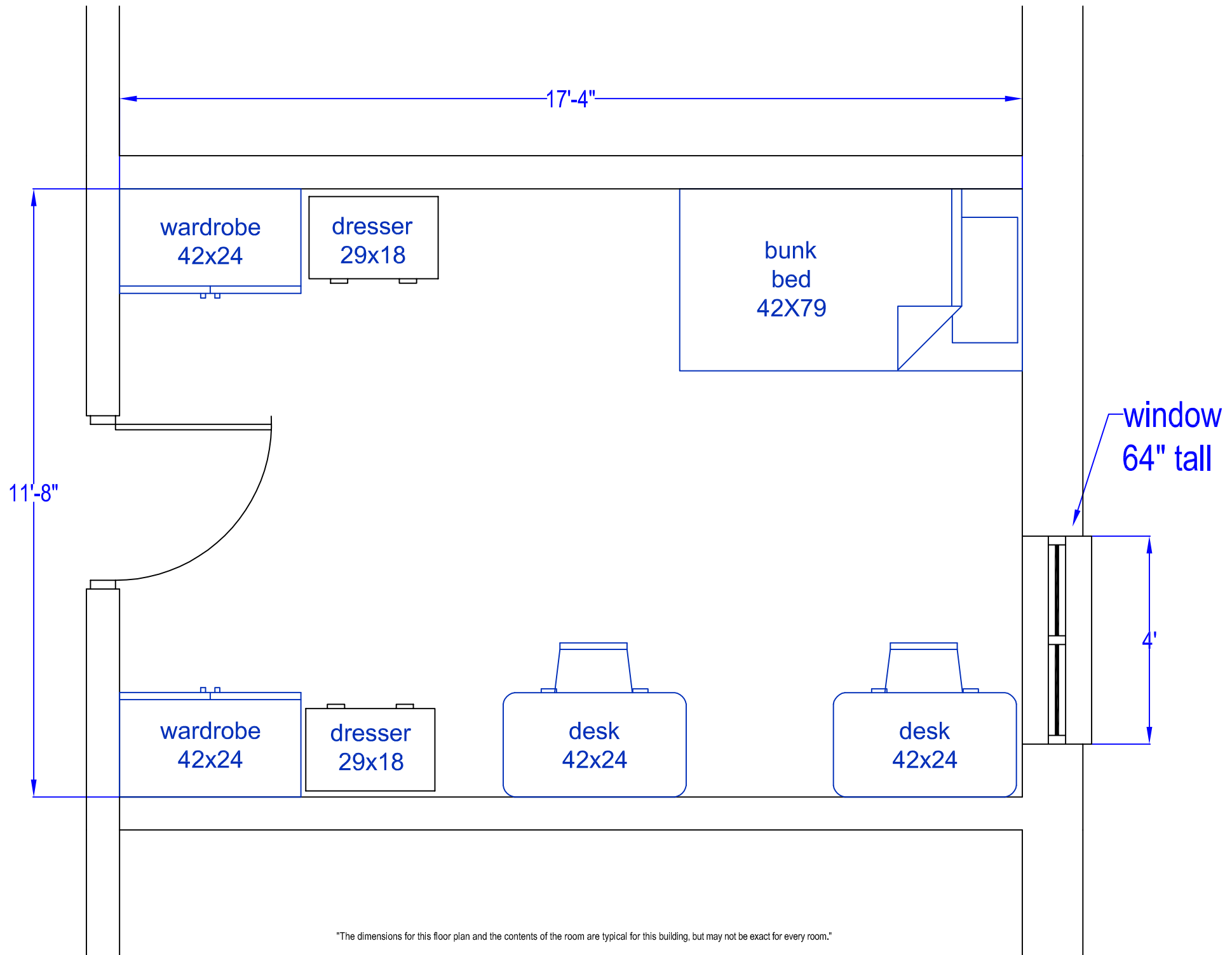
McKinney and McChesney typical room.
